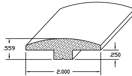
DWG #473 T-MOLDING
