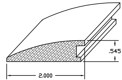
DWG #706 REDUCER
