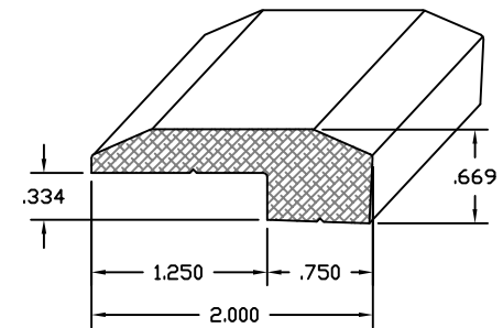
DWG #474 THRESHOLD
