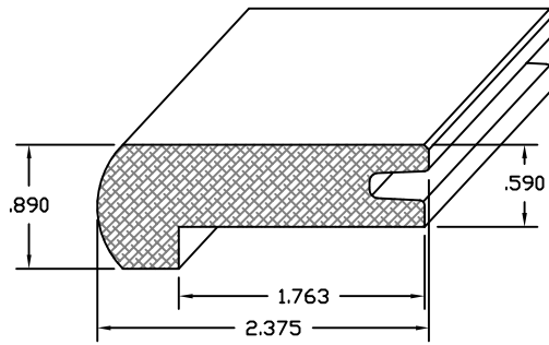
DWG # 715 STAIRNOSE
