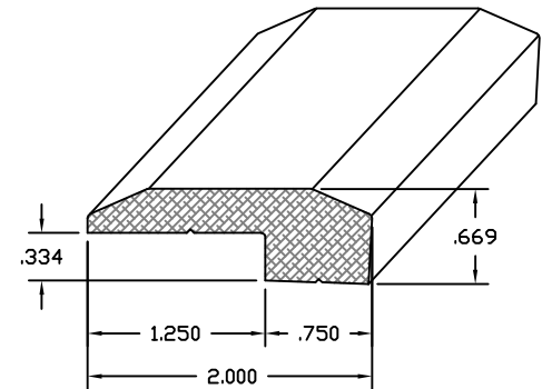
DWG #474 THRESHOLD
