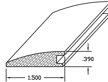
DWG # 701 REDUCER
